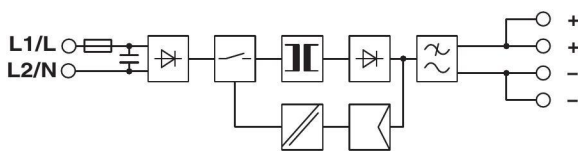
Figure 2 Block diagram
