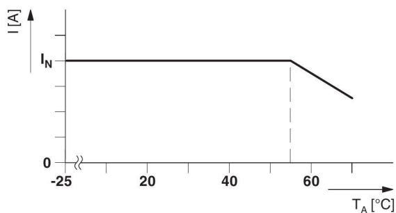
Figure 14 Temperature-dependent derating
